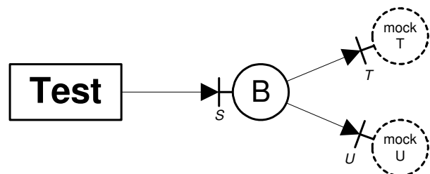
Figure 3. Iterative Interface Discovery
